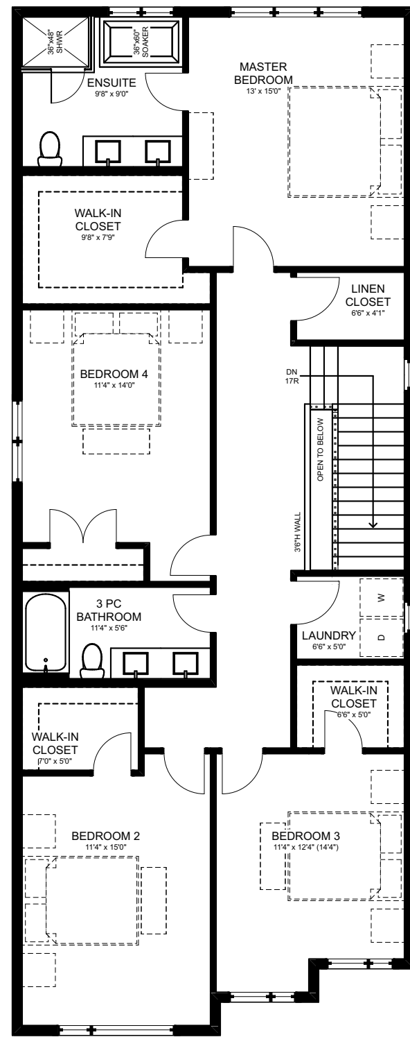
SECOND FLOOR - 9' CEILING 1,444.6 sq ft
